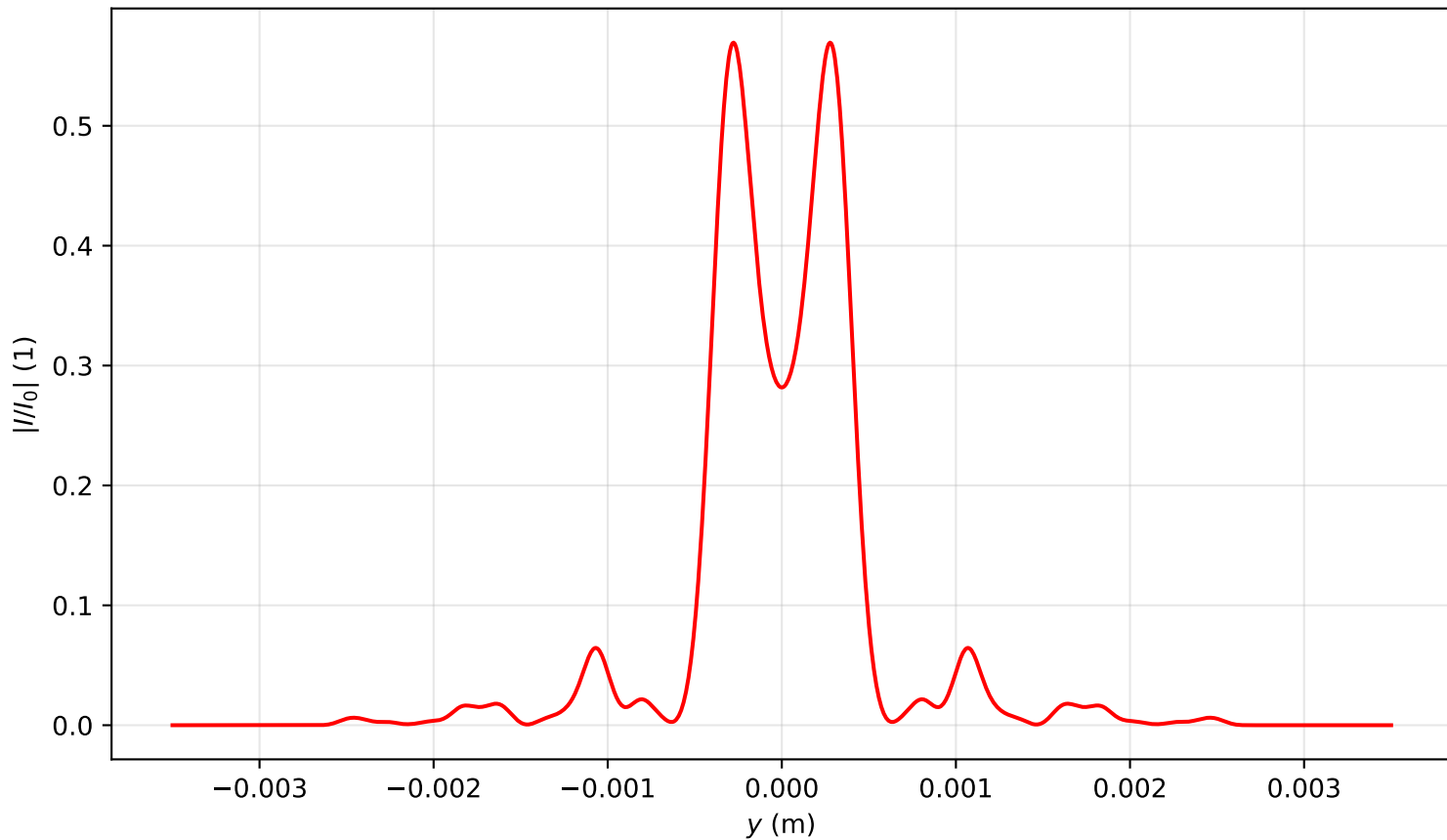
Intensity profile I(x=0, y, z=2.149)/I_0 , P_{in}=4.5P_{cr} , artificial time
